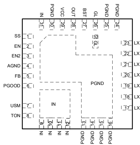
AOZ2295AQI-03 31-Pin 4mm x 4mm QFN
