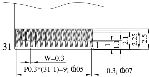
FPC Contact Side SCALE 1:2.5
