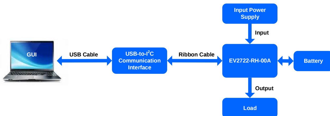
Figure 1: EVKT-MP2722 Evaluation Kit Set-Up
