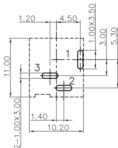
Recommended PCB Layout Bottom View
