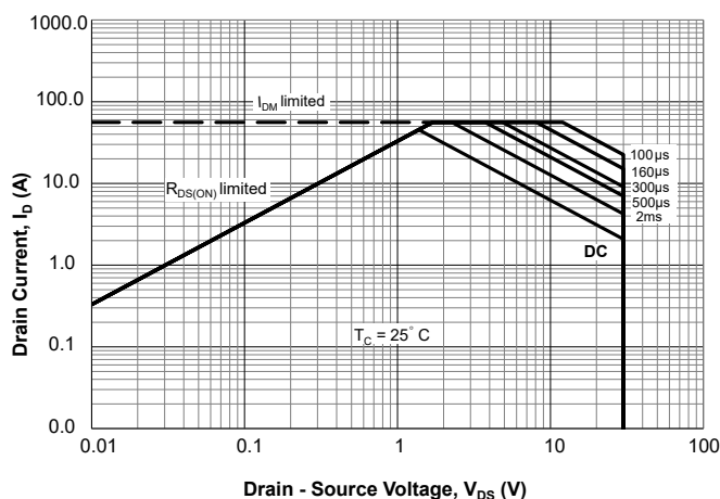
Figure 10. Safe Operating Area (SOA) Curves for Power Switch
