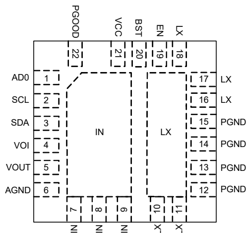
22-Pin 4mm x 4mm QFN (Top View)
