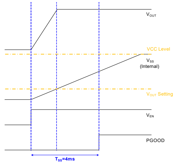
Figure 5. Soft-Start Sequence of AOZ2233CQI-24
