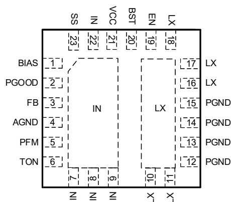
AOZ2221QI 23-pin 4mm x 4mm QFN
