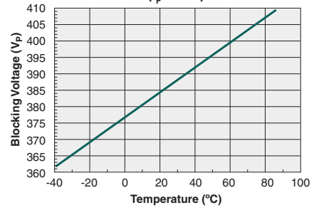
Form-B Typical Blocking Voltage vs. Temperature ( I_F=5mA )
