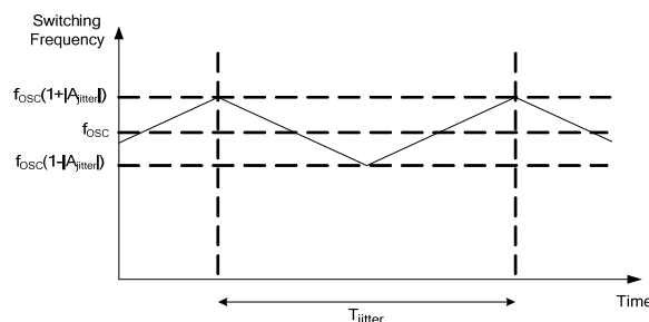
Figure 3: Frequency Jittering
