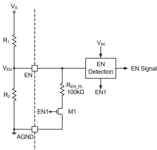
Figure 6. Enable Internal Circuit
