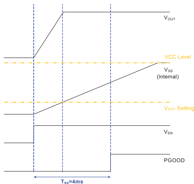
Figure 5. Soft Start Sequence of AOZ22701QI
