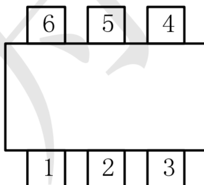
Pin Configuration
