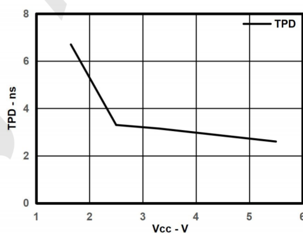
Fig. 8-2. TPD Across V_{CC} at 25°C
