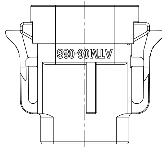
P/N ATM06-08SB-SF1BK KEY-B CONFIGURATION STANDARD COLOR: BLACK
