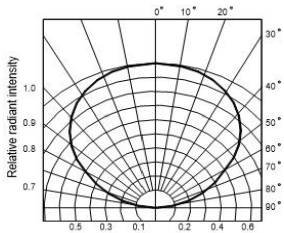
Fig.6 Radiation diagram
