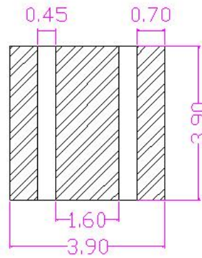
建议焊盘尺寸: Recommended Soldering Pattern
