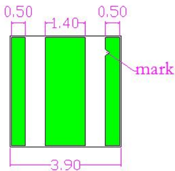
建议焊盘尺寸: Recommended Soldering Pattern
