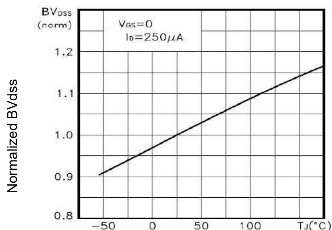
TJ-Junction Temperature(°C) Figure 9 BVdss vs Junction Temperature
