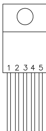
TO220T-5
