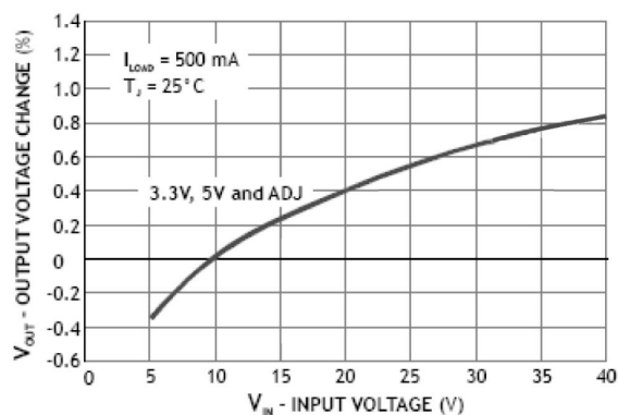
LINE REGULATION
