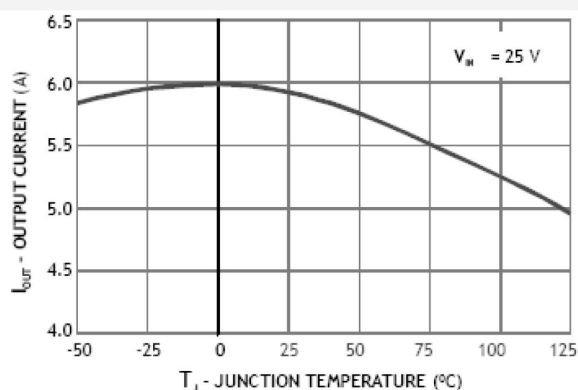
CURRENT LIMIT
