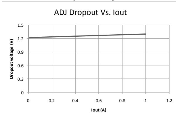
Dropout Voltage
