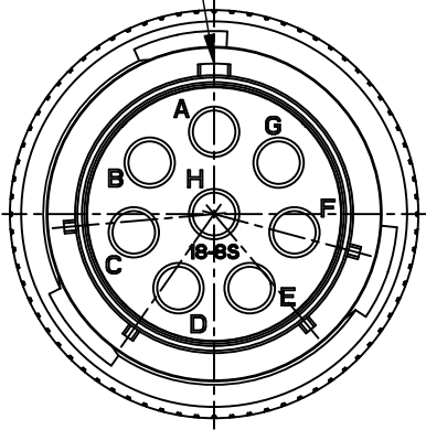
MASTER KEYWAY
