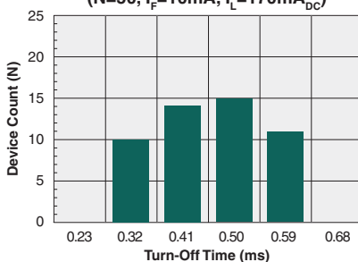
Form-A Typical Turn-Off Time (N=50, I_F=10\text{mA} , I_L=170\text{mA}_{\text{DC}} )
