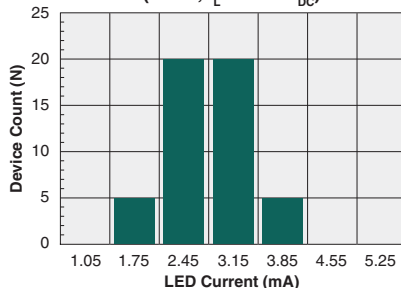
Form-A Typical I_F for Switch Dropout (N=50, I_L=170\text{mA}_{\text{DC}} )
