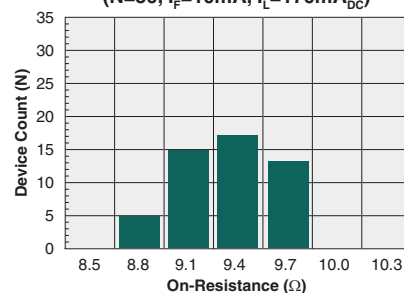
Form-A Typical On-Resistance Distribution (N=50, I_F=10\text{mA} , I_L=170\text{mA}_{\text{DC}} )
