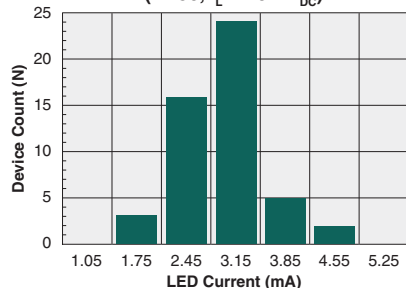
Form-A Typical I_F for Switch Operation (N=50, I_L=170\text{mA}_{\text{DC}} )
