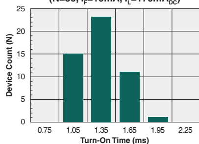
Form-A Typical Turn-On Time (N=50, I_F=10\text{mA} , I_L=170\text{mA}_{\text{DC}} )
