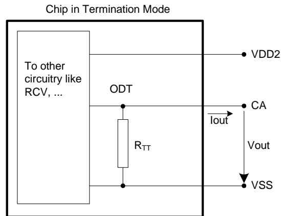
Figure - CA On Die Termination
