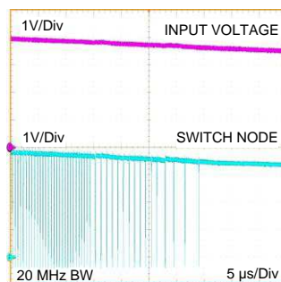
Figure 40. High duty cycle operation and switching frequency reduction.
