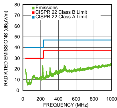
Figure 3. Radiated EMI (CISPR22) V_{IN} = 5.0V , V_{OUT} = 1.8V , I_{OUT} = 650mA
