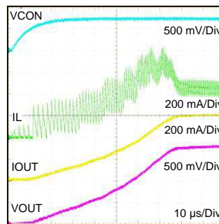
Figure 38. Startup behavior of current limit based softstart.
