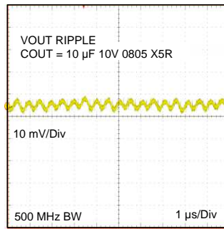
Figure 2. Output Voltage Ripple V_{IN} = 5.0V , V_{OUT} = 1.8V , I_{OUT} = 650mA
