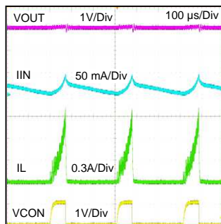
Figure 39. Hiccup behavior with persistent output short circuit.
