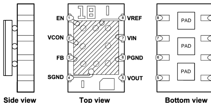
Figure 4. Package Number NQB0008A
