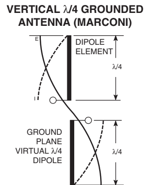
Figure 26: Dipole Antenna
