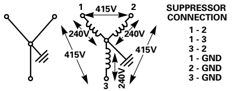
FIGURE 25F. 3 PHASE 240V/415V
