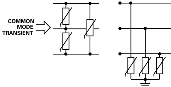
FIGURE 26A. INCORRECT FIGURE 26B. CORRECT FIGURE 26. COMMON MODE TRANSIENT AND CORRECT SOLUTION
