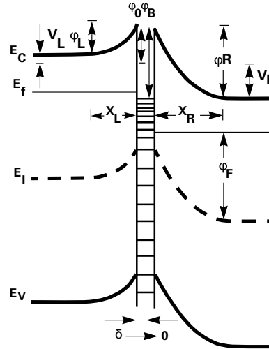
FIGURE 5. ENERGY BAND DIAGRAM OF A ZnO-GRAINBOUNDARY-ZnO JUNCTION
