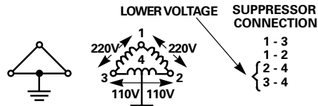
FIGURE 25D. 3 PHASE 220V
