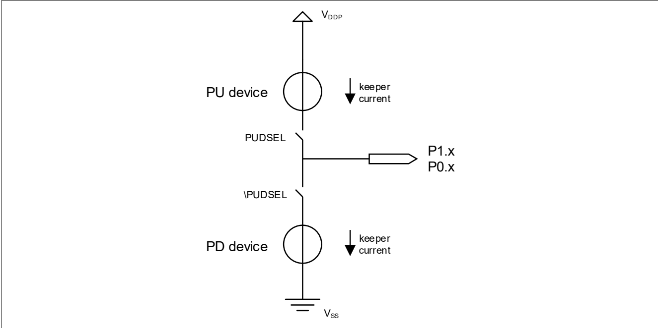
Figure 32 Pull-up/down device
