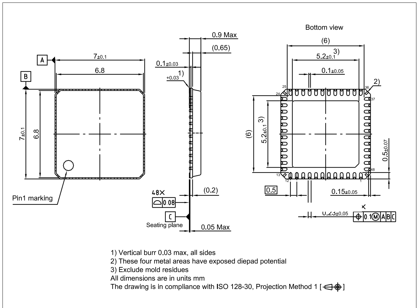
Figure 36 Package outline VQFN-48-31 with LTI (BF step) 1)
