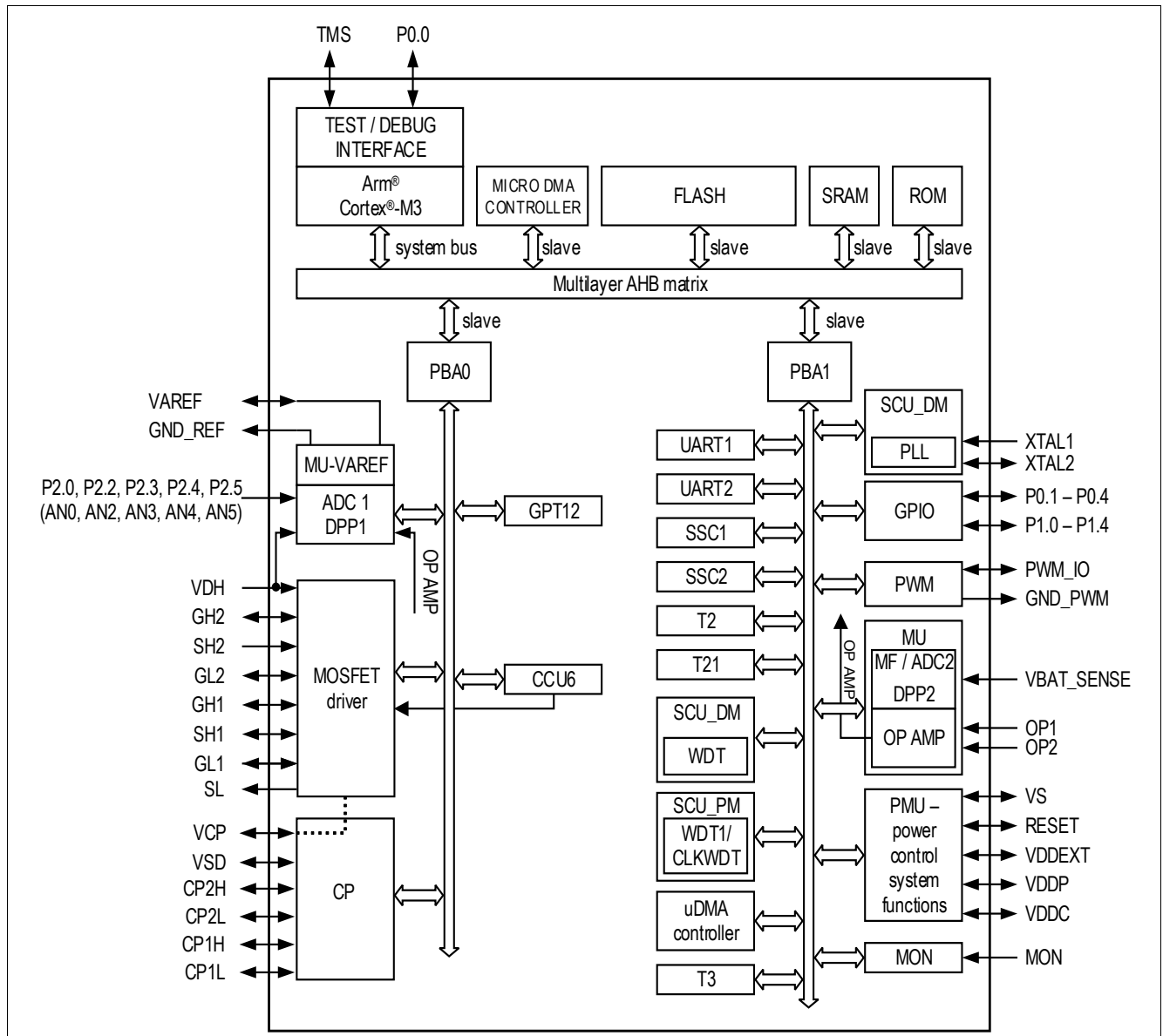
Figure 1 Block diagram
