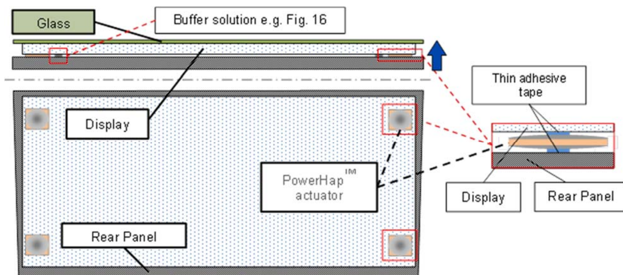
Fig. 15: Schematic drawing of a possible user application of the PowerHap actuator for generating a haptic feedback onto a touchscreen panel display
