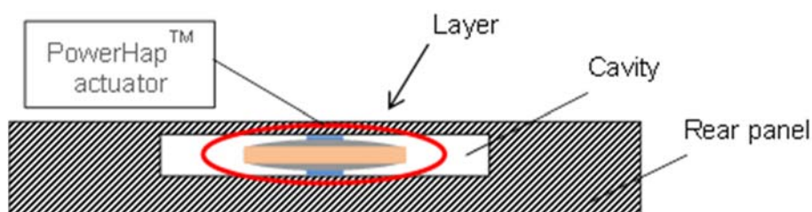
Fig. 13: Schematic Illustration using the PowerHap™ actuator underneath a thin and flexible layer, e.g. implementation underneath buttons.
