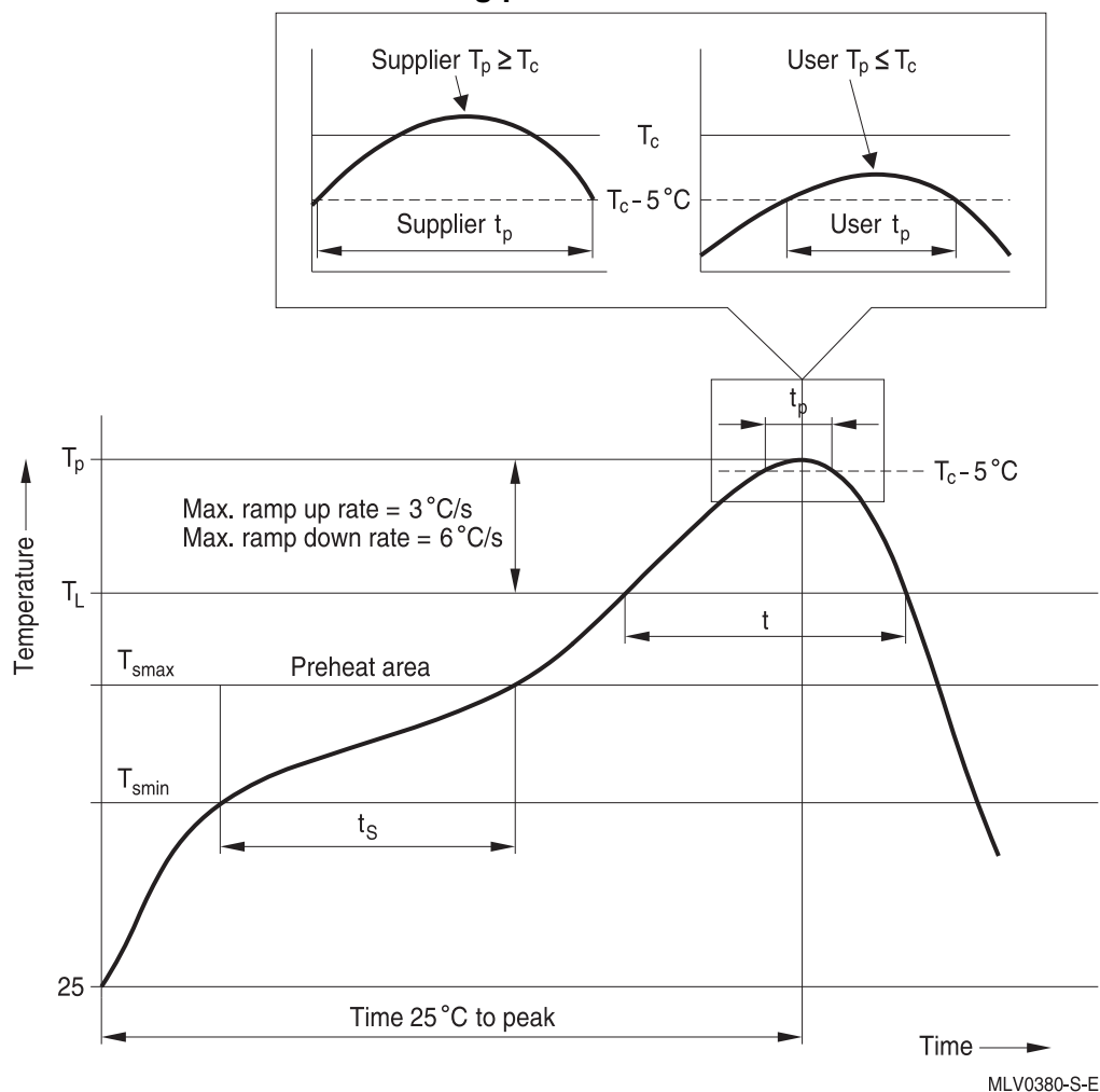
Fig. 11: Reflow soldering profile
