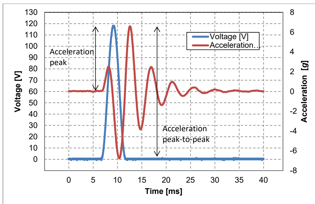
Fig. 5: Typical acceleration as a function of input voltage with 100 g load. Input voltage with a half wave sinus signal form of amplitude 0 to 120 V and pulse length 5ms which is equivalent to 200 Hz.
