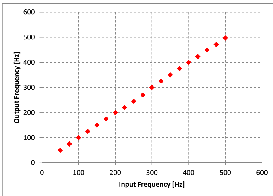
Fig. 8: Output frequency of acceleration vs. input voltage signal frequency for 10 pulses. Input voltage has a single pulse half wave sinus signal form of amplitude 0 to 120 V and varying frequency from 50 to 500 Hz. The frequency of output acceleration is calculated.
