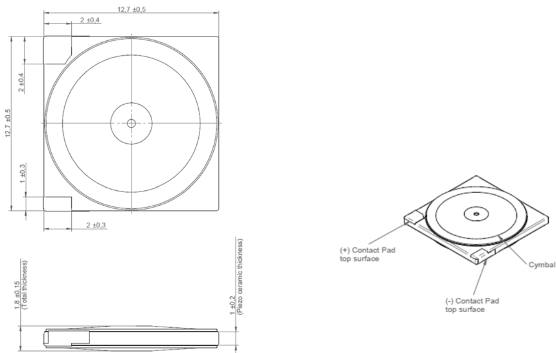
Fig. 1: Dimensional drawings
