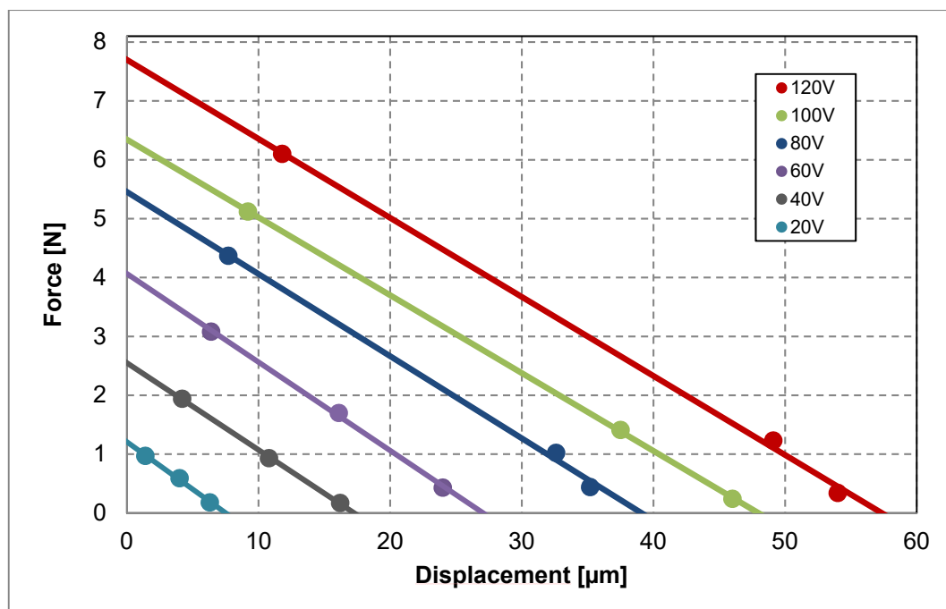
Fig. 3: Force-stroke diagram with different load springs. Typical stiffness 130N/mm.
