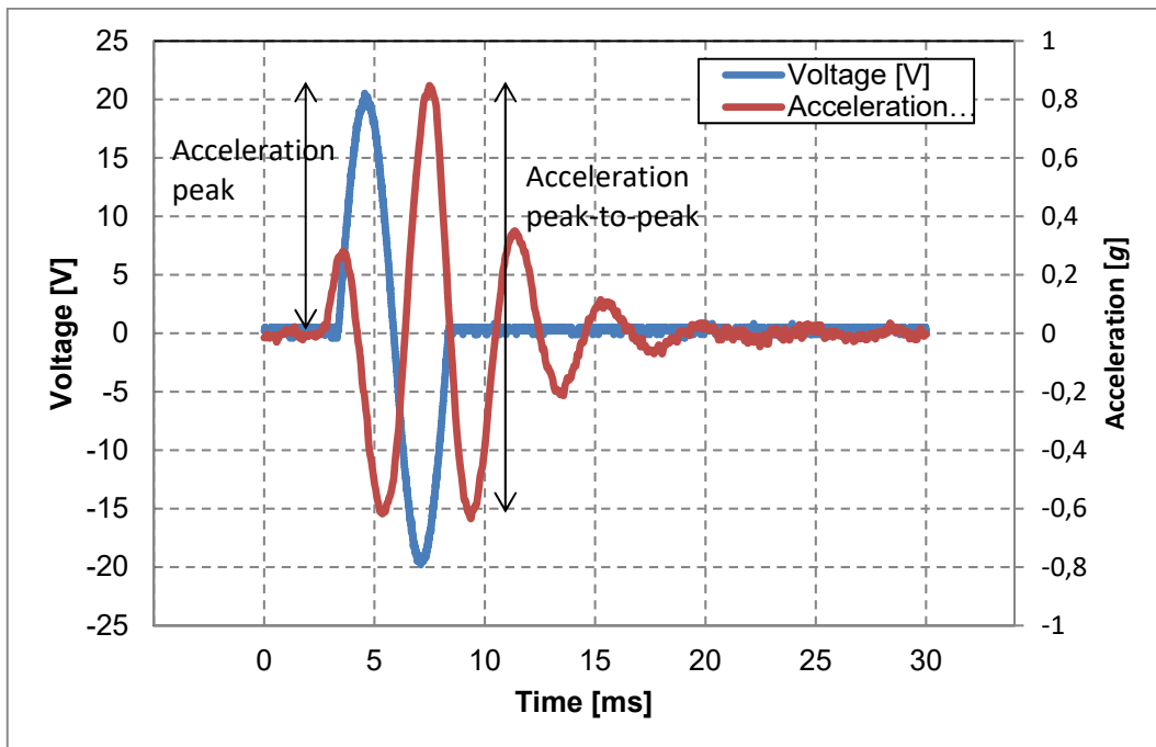
Fig. 6: Typical acceleration as a function of input voltage with 100 g load. Input voltage with a sinus signal form of amplitude -20 to 20 V and pulse length 5ms which is equivalent to 200 Hz.
