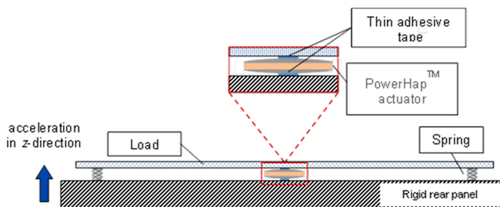
Fig. 14: Schematic drawing of a simplified setup involving the usage of springs to ensure the movement of a non-flexible load in z-direction.
