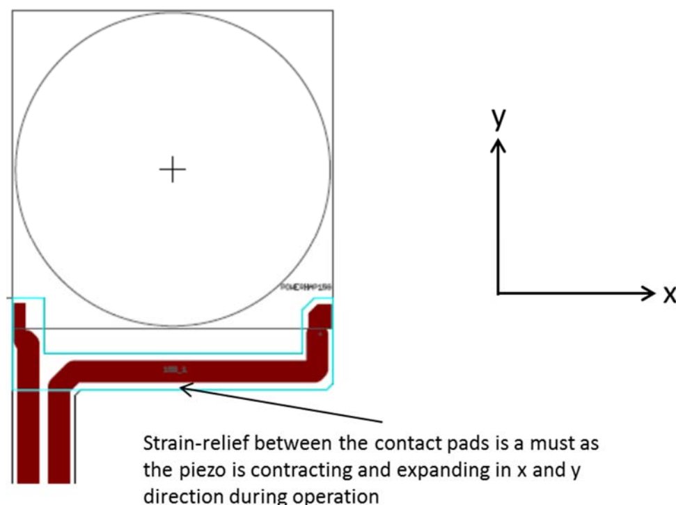
Fig. 12: Example of PowerHap with flexible PCB contact element.
