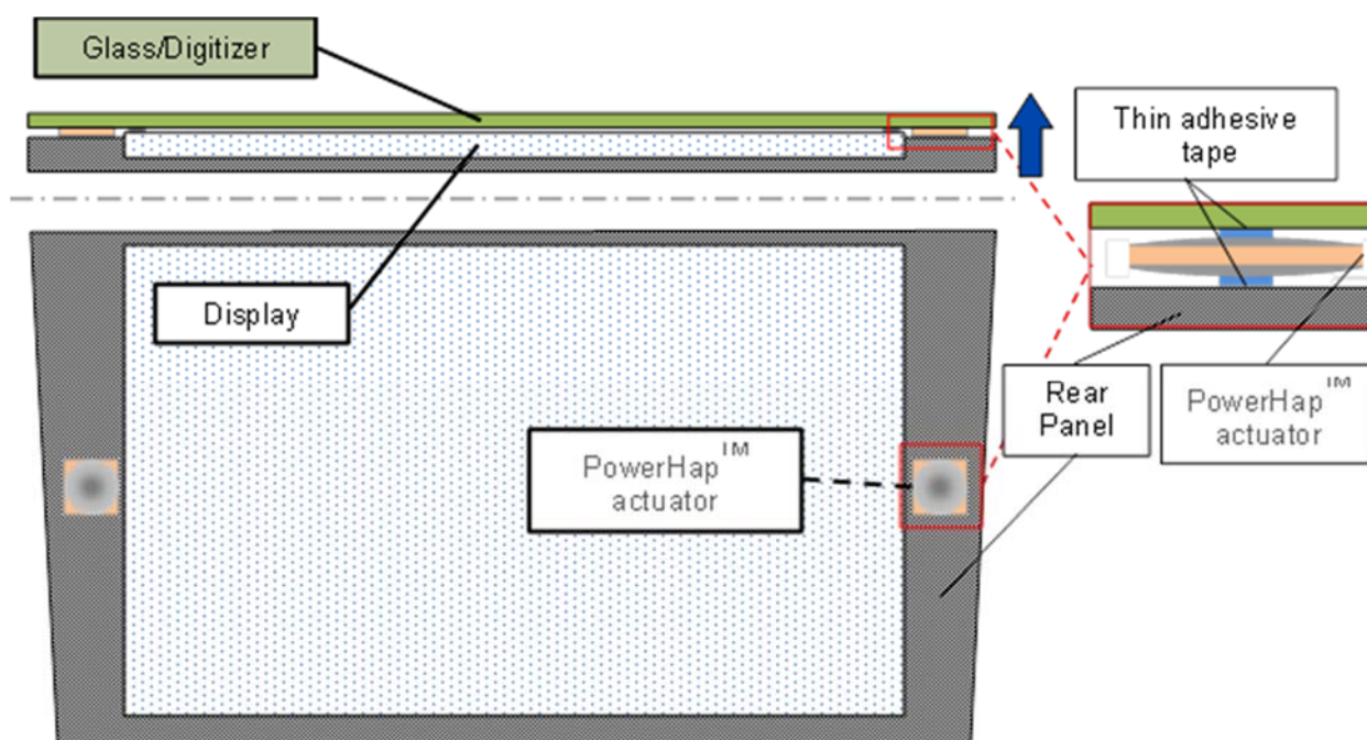
Fig. 17: Schematic drawing of a possible user application of the PowerHap actuator for generating a haptic feedback onto the digitizer of a display.
