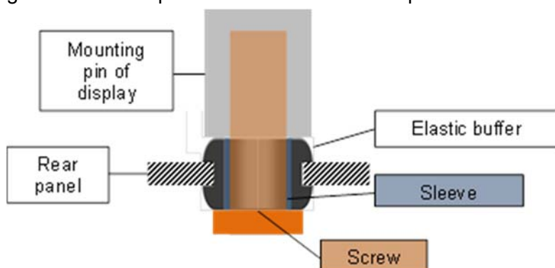
Fig. 16: Schematic drawing of a potential option for a buffer that is able to ensure movement x,y- and z-direction depending on the material and the dimension of the elastic buffer used.
