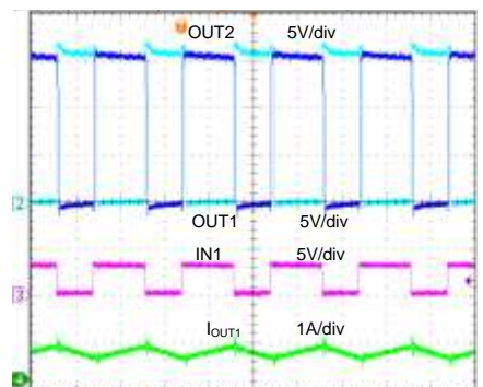
Operation Waveform (VCC=VM=16V, I o =0.5A, IN2=IN1)
