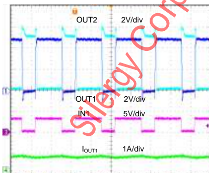
Operation Waveform (VCC=VM=5V, I o =0.5A, IN2=IN1)
