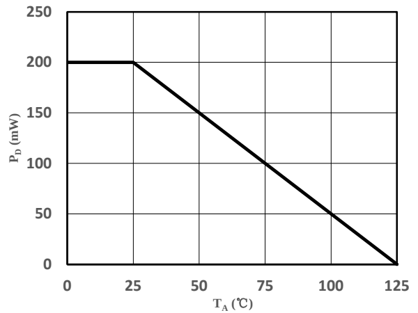
Fig 4 Derating Curve
