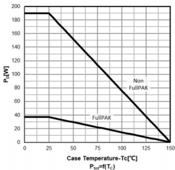
Power dissipation
