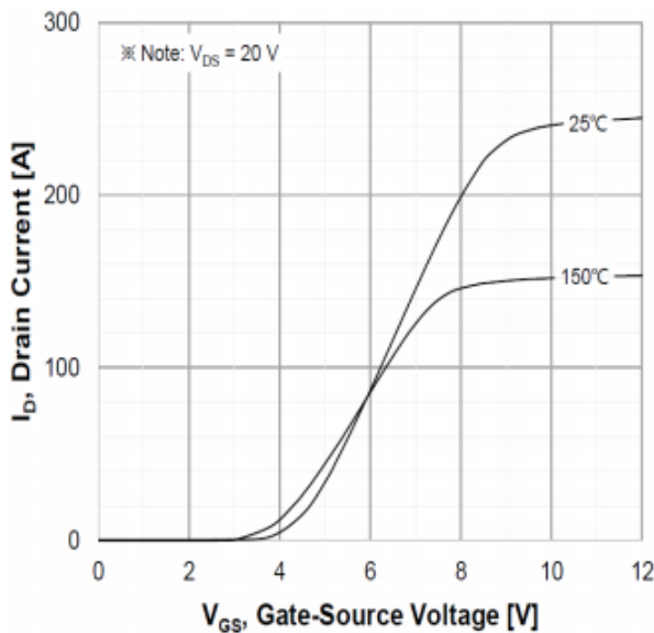
Transfer characteristics
