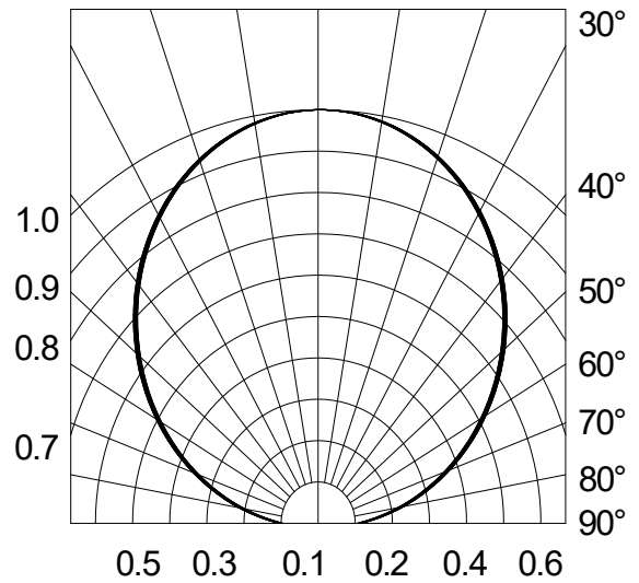
Fig.6-Radiation Diagram T a =25°C
