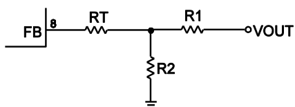
Figure 6: T-Type Network
