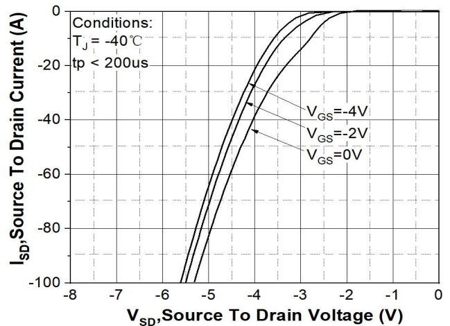
Figure 8. Body diode characteristic at T_J = -40^\circ\text{C}
