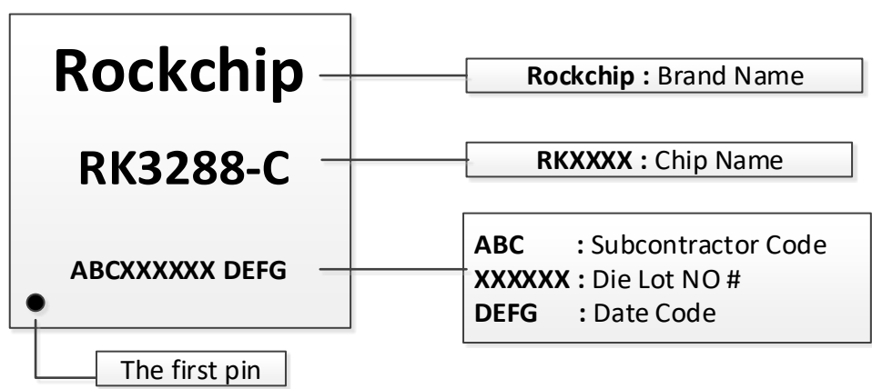
Fig. 2-2 RK3288 W Version Silk Marking
