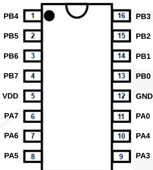
PFC154-S16: SOP16 (150mil) PFC154-D16: DIP16 (300mil)
