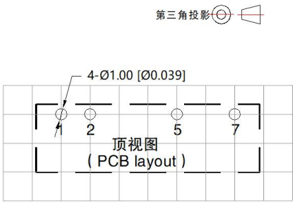
注: 栅格距离 2.54*2.54mm
