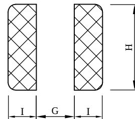
( PCB Pattern )
