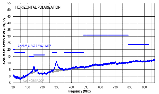
CISPR25 Class 5 Average Radiated Emissions Horizontal, 30MHz to 1GHz
