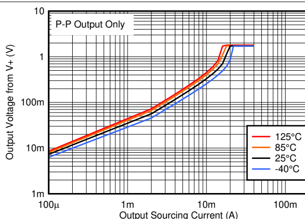
Figure 6-8. Output Sourcing Current vs. Output Voltage, 1.8V
