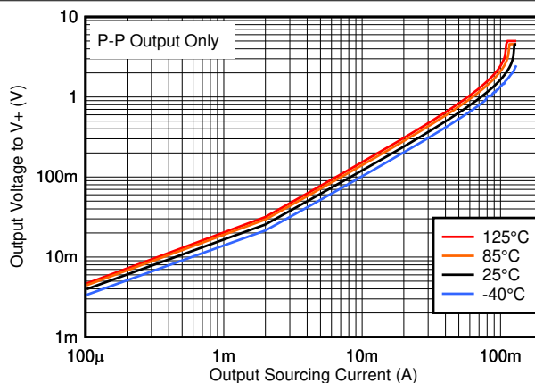
Figure 6-12. Output Sourcing Current vs. Output Voltage, 5V
