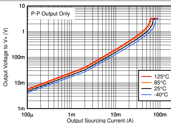
Figure 6-10. Output Sourcing Current vs. Output Voltage, 3.3V
