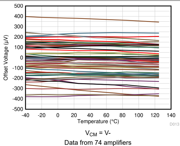
Figure 6-3. Offset Voltage vs Temperature
