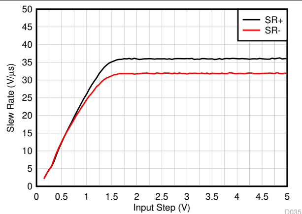
Figure 6-11. Slew Rate vs Input Step Voltage
