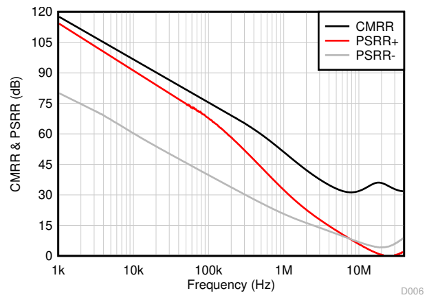
Figure 6-16. CMRR and PSRR vs Frequency
