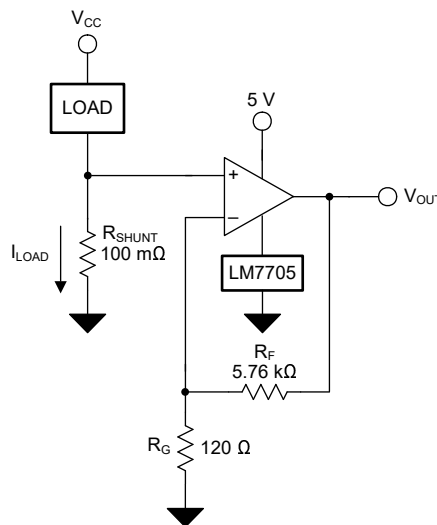
Figure 8-1. TLV936x-Q1 in a Low-Side, Current-Sensing Application
