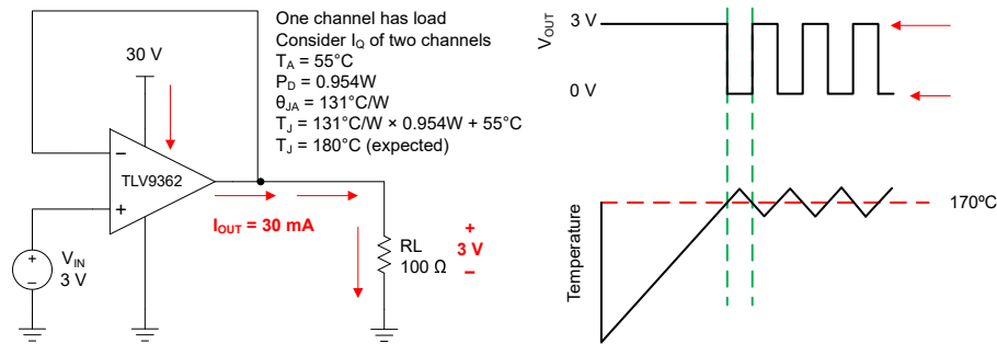
Figure 7-2. Thermal Protection
