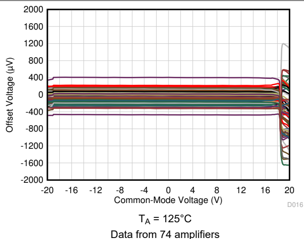
Figure 6-5. Offset Voltage vs Common-Mode Voltage
