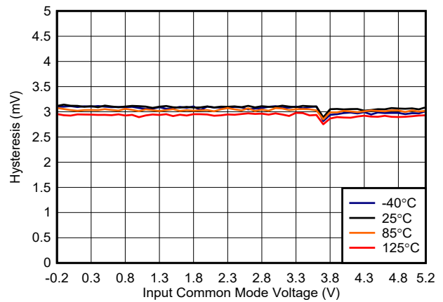
Figure 6-10. TLV3601 Hysteresis vs. Common-Mode, 5 V
