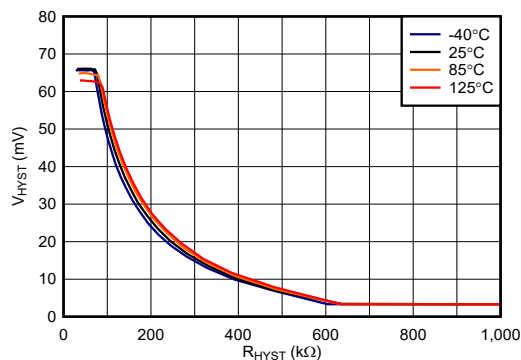
Figure 8-2. V_{\text{HYS}} (mV) vs R_{\text{HYS}} (kΩ), V_{\text{CC}} = 5\text{ V}
