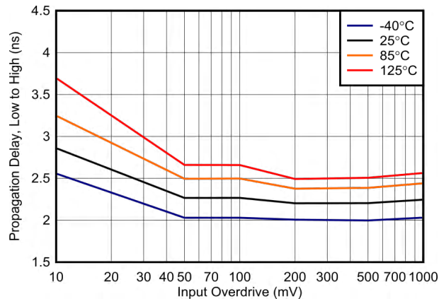
Figure 6-43. Propagation Delay, Low to High, 5 V
