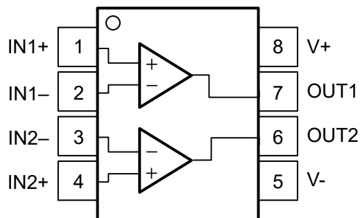
Figure 5-3. TLV3602 DKG, DSG Packages 8-Pin VSSOP, WSON
