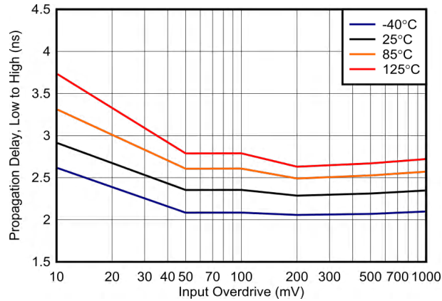
Figure 6-41. Propagation Delay, Low to High, 3.3 V
