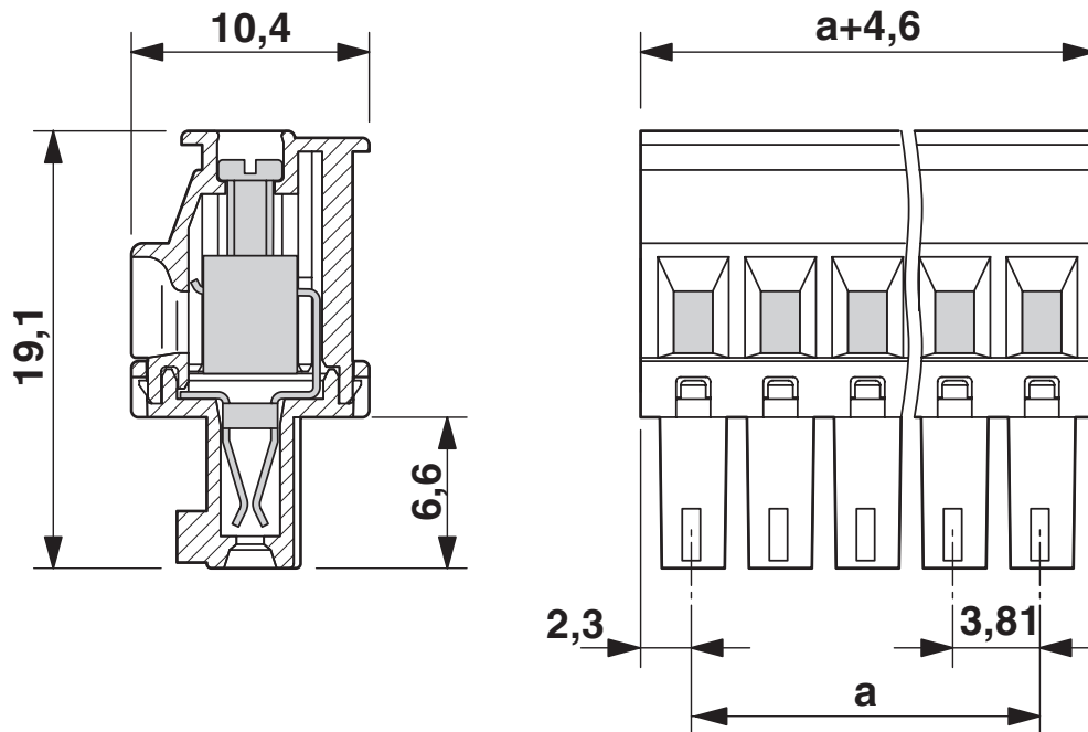
Dimensional drawing
