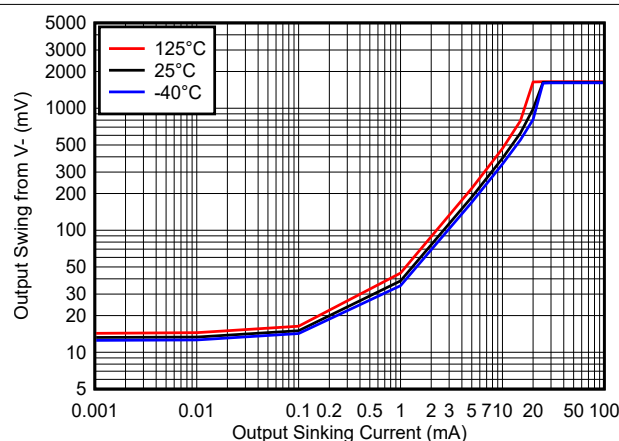
Figure 8-1. Output Swing vs. Output Sinking Current - 1.8V
