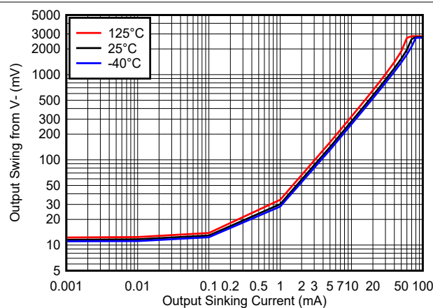
Figure 8-3. Output Swing vs. Output Sinking Current - 3.3V
