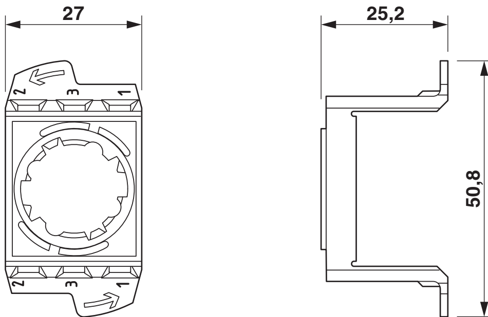
Dimensional drawing
