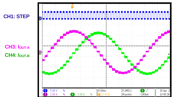
1/8 Microstepping
