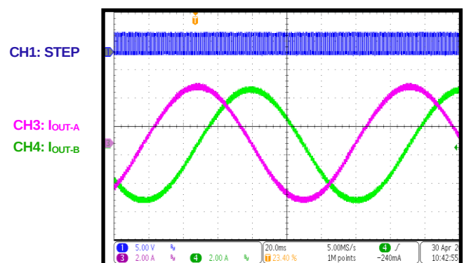
1/32 Microstepping
