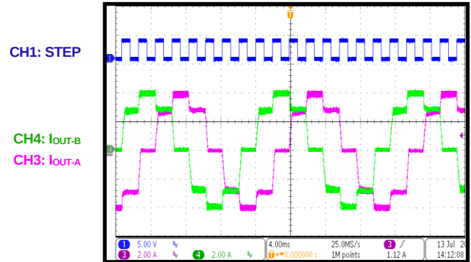
Half-Step
