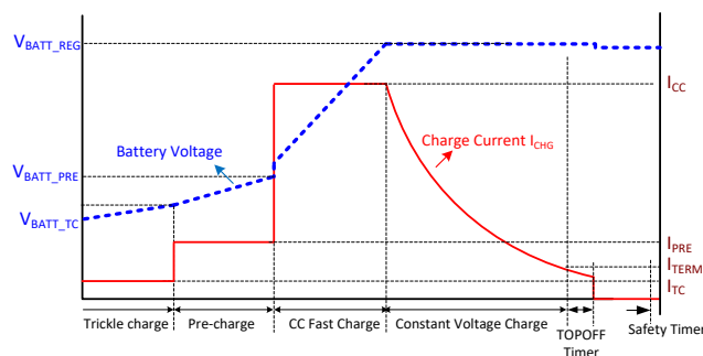
Figure 4: Battery Charging Profile
