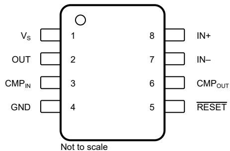
Figure 5-1. INA310x: DGG Package 8-Pin VSSOP Top View
