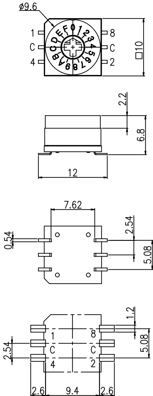
Recommended PCB Layout Top View
