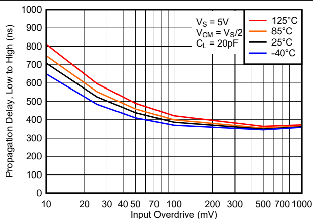
Figure 7-14. Propagation Delay, Low to High, 5 V
