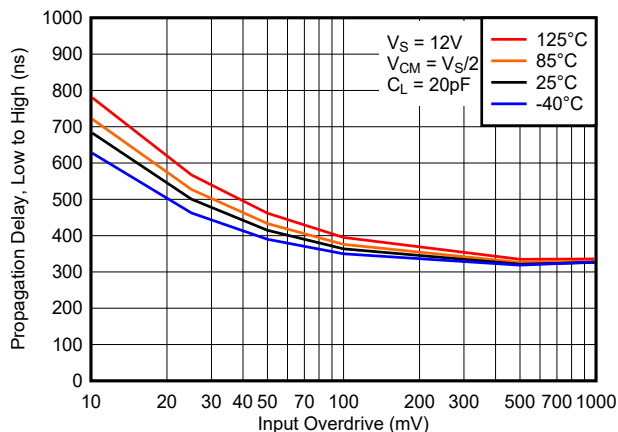
Figure 7-16. Propagation Delay, Low to High, 12 V
