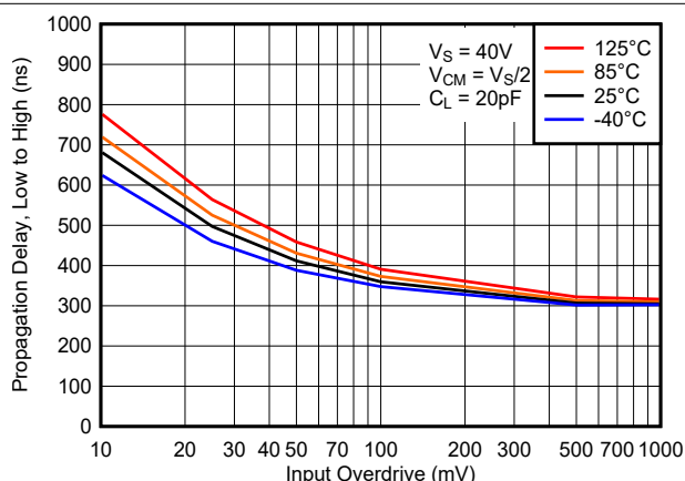
Figure 7-18. Propagation Delay, Low to High, 40 V
