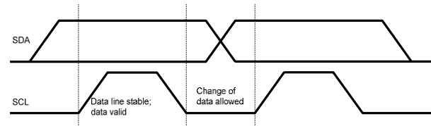
Figure 5: Bit Transfer on the I 2 C Bus
