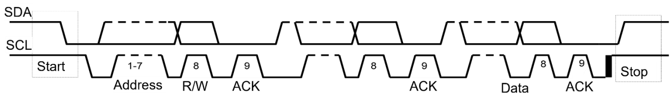
Figure 7: Complete Data Transfer
